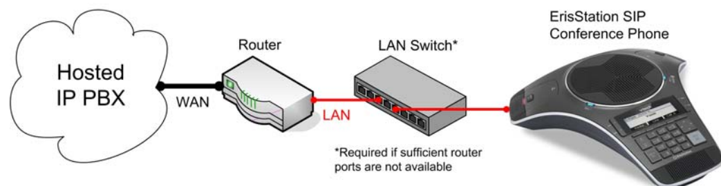
Figure 1. VCS752 Installation Example
